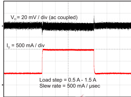
Figure 28. TPS562209 Transient Response
