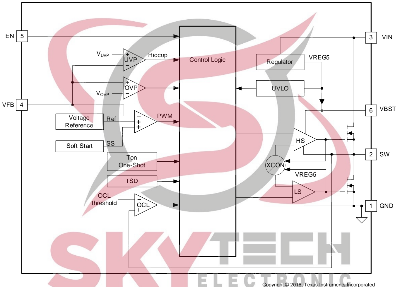
Figure 19. TPS56x209
