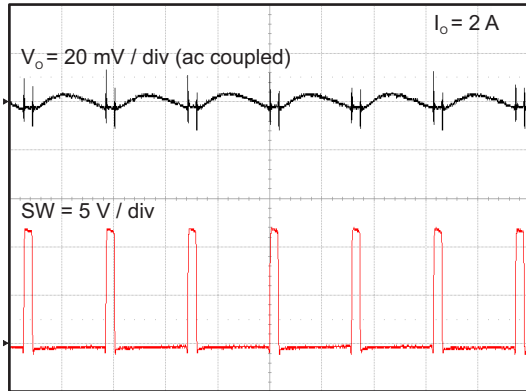
Figure 27. TPS562209 Output Voltage Ripple
